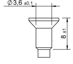
Alternatively at countersunk heads: modification of the shank at drilled head
