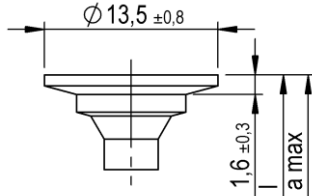
Large washer head II
