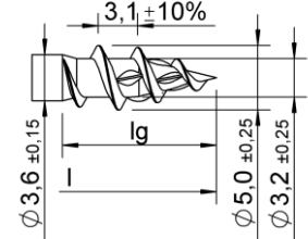
Grobgang II
