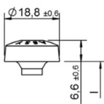
Pan Head
