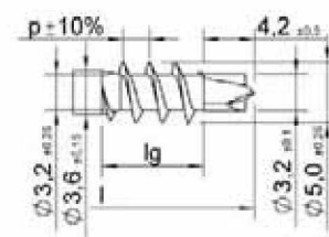
ASSY plus 3,0
