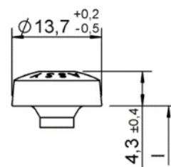
Pan Head
