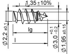
single – threaded
