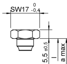
Kombi hexagonal head with and without collar
