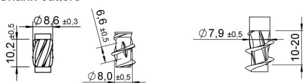
Shank cutters
