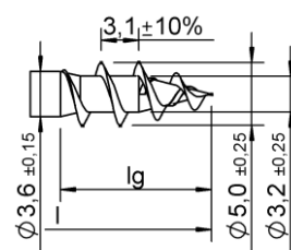
Groggang I
