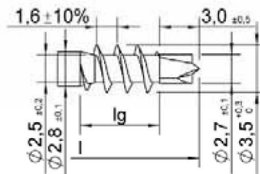
ASSY plus 3,0
