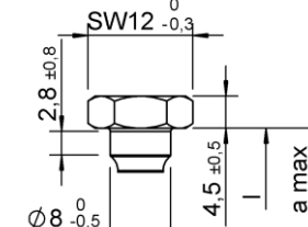
Kombi hexagonal head with and without collar
