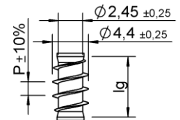
Underhead thread Lg2 < 4 x d, P= 1.8, 2.2
